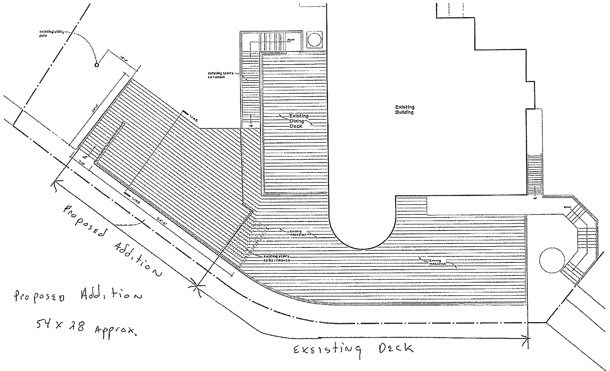
1 Proposed Deck Plan 1/8" = 1'-0"
